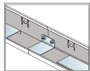
Detail of Thinline splice
